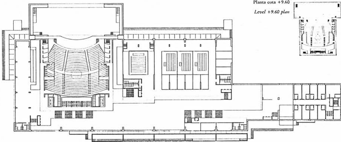
Planta cota +6.40 / Level +6.40 plan
